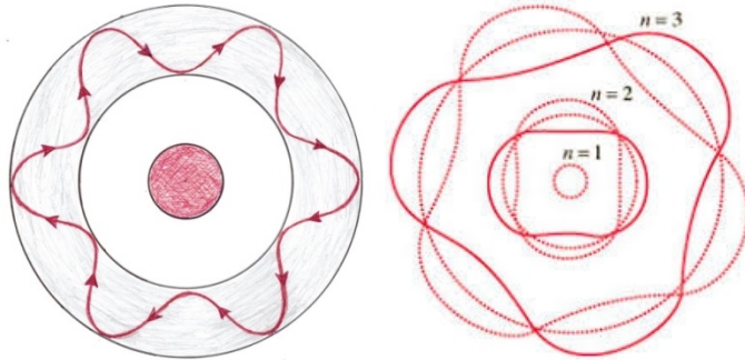
Graphical representation of elementary particle
