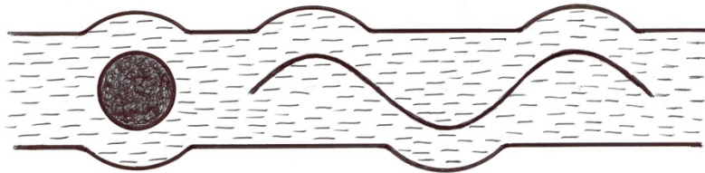
Solid-state of particle
