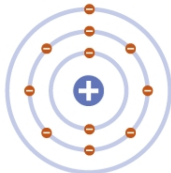
graphical representation of atom
