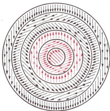
This is the fine space layers of the atomic structure
