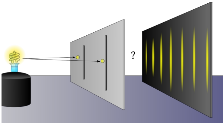
Double slit experiment
