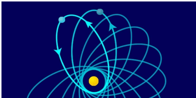
This is the precession (not regression) of Mercury orbit which Theory of Relativity actually predicting
