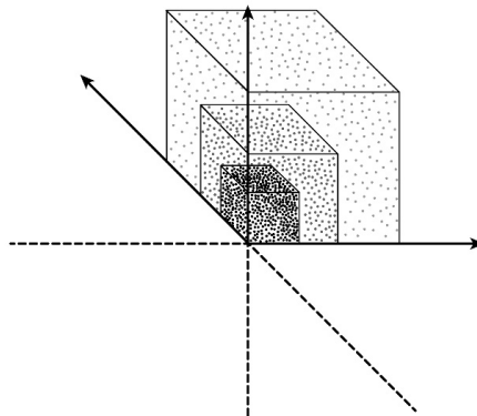
3D vectors producing only 1/8 of Space volume and continuous (catastrophic)distortional expansion
