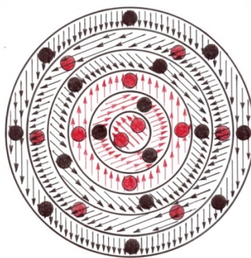
Shell configuration of atomic nucleus where the neutrons are separating the proton shells
