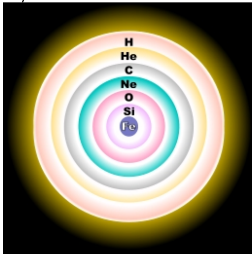
This is the sequence of how the elements suppose to be produced in the Stars
