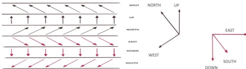
The fine space layers and their opposing orientations
