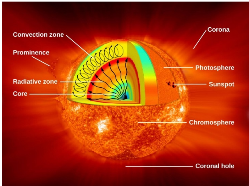
This is our current model of the Sun
