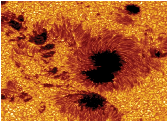
Photo of Sun surface and its cooler interior.
