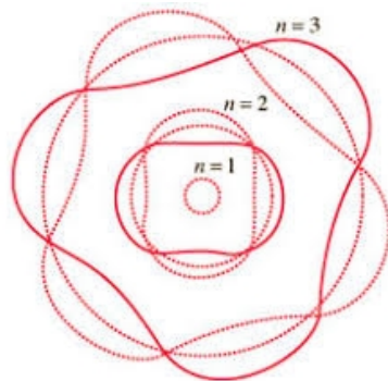
The harmonic resonance of atom's waves
