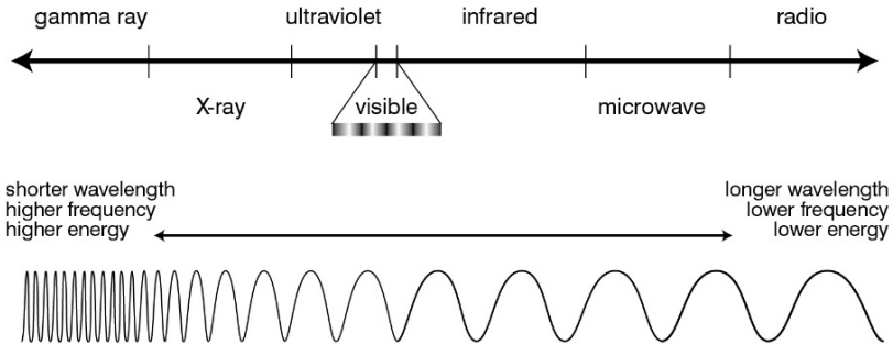
Diagram of the electromagnetic spectrum (the visible light is just small part)
