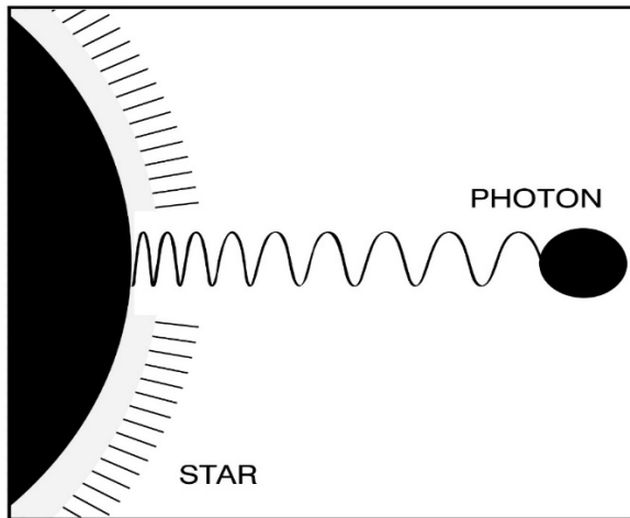
Gravitational red-shift
