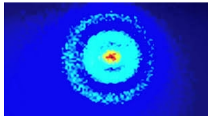
Photo of the Hydrogen atom
