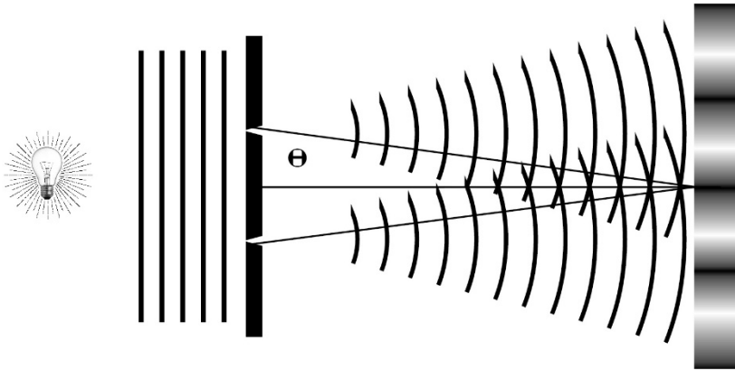
Double slit experiment
