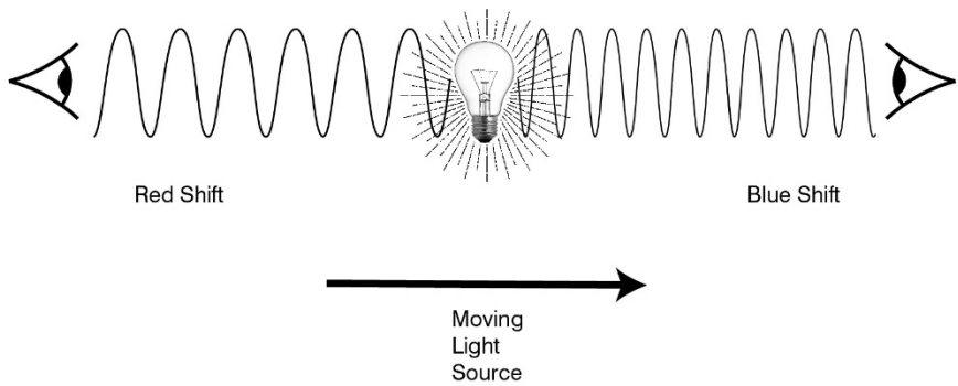
Light redshift effect of moving source
