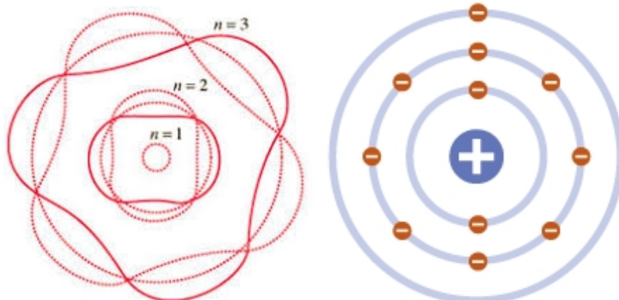
The harmonic resonance of atoms waves
