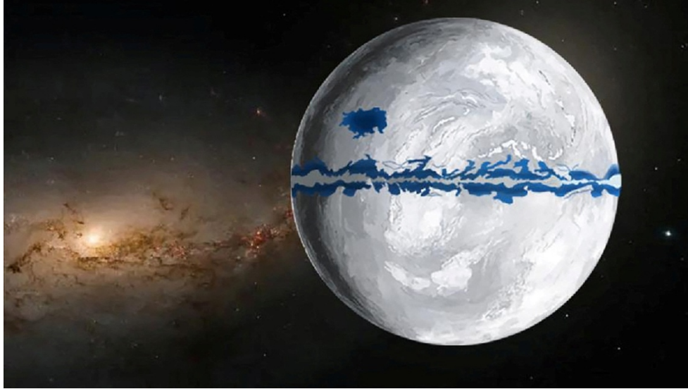
This is how was looked Earth when the concentration of CO 2 was low
